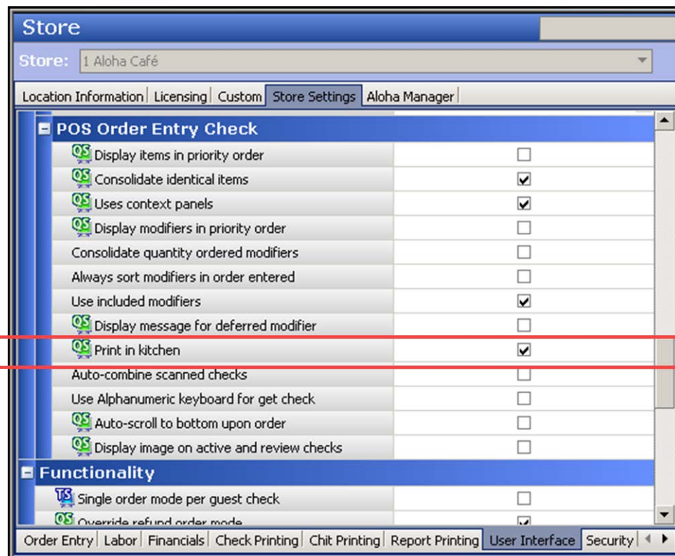
Figure 41 Store - Store Settings tab - User Interface group
