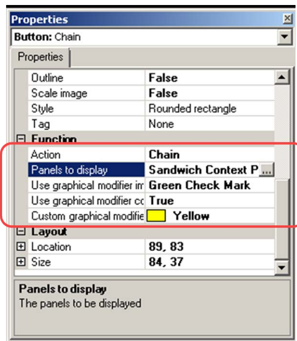
Figure 36 Chain button function
