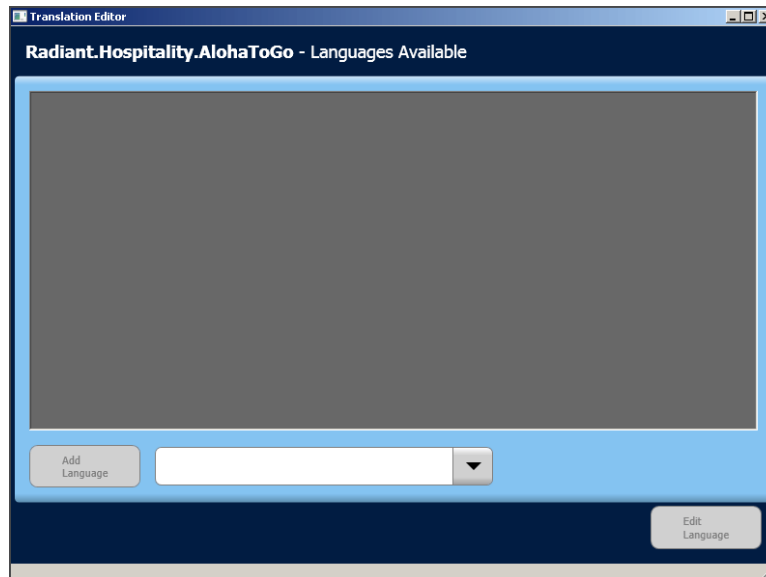
Figure 8 Translation Editor
