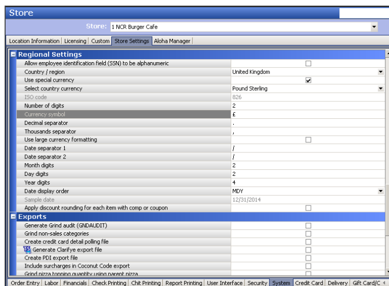
Figure 4 Regional Settings
