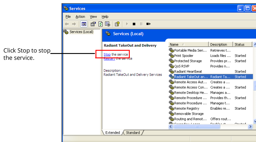
Figure 6 Services
