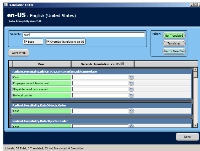
Figure 14 Search Results
